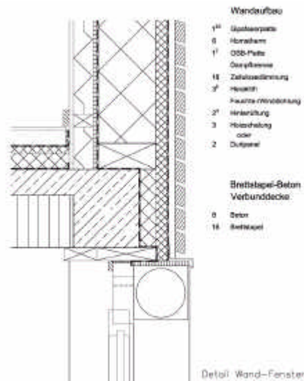
Abb. 13 Block 9 Detail Wand- Fenster
